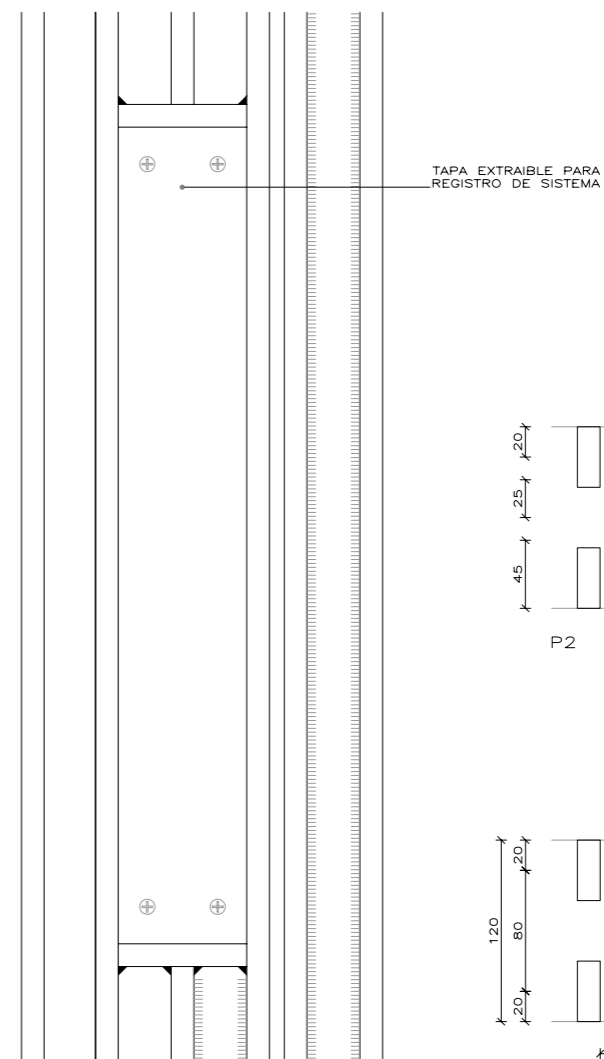
ALZADO INTERIOR
